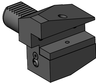
90DEG VDI30 STATIC TOOL OUTPUT: 3/4" SQR SHANK COOLANT: EXTERNAL
